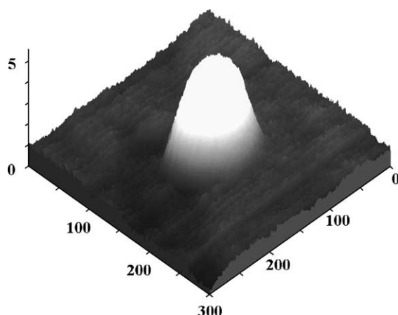
Fig. 3. UHV AFM contact mode image of sapphire (Al 2 O 3 , c-plane 0001) bombarded with 500 eV Ar 7+ ions. Nanodefects induced by these ions with same kinetic but higher potential energy as compared to Ar + ions (see Fig. 2) are considerably higher and wider than the ones caused by singly charged ions. All dimensions in nanometers.
